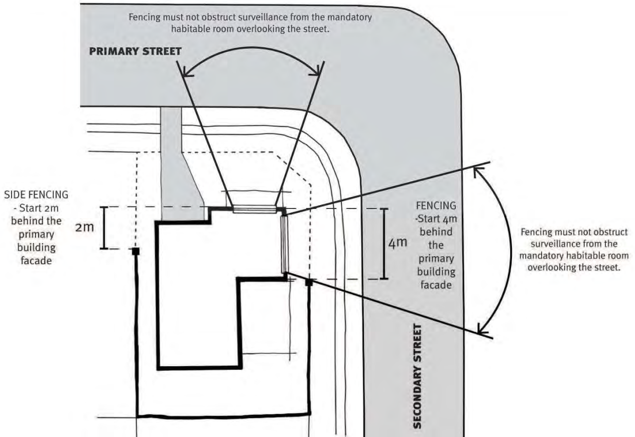
Figure 4-12 Fencing Design
