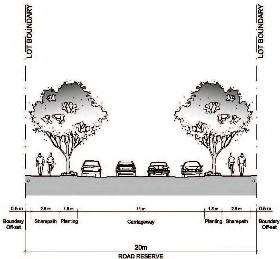
Figure 3-12: Typical collector road (off road cycle path)
