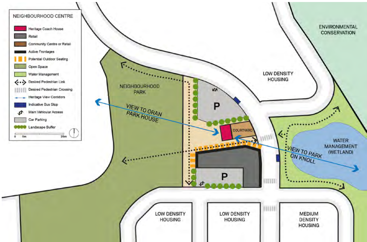
Figure 3-2: Indicative Layout of Coach House Neighbourhood Centre
