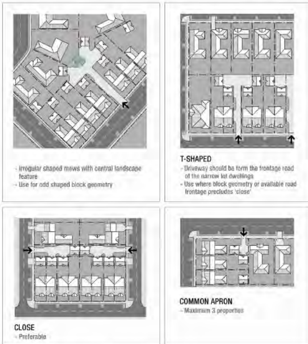
Figure 3-19: Indicative examples of shared driveways
