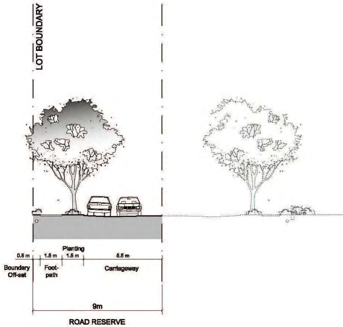
Figure 3-20 Temporary half road width construction
