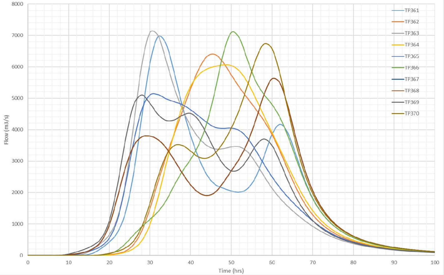
ARR16 Rainfall ARR87 Losses - 48 Hour Event Figure 7 1% AEP IFD Comparison at Nepean at Gulger
