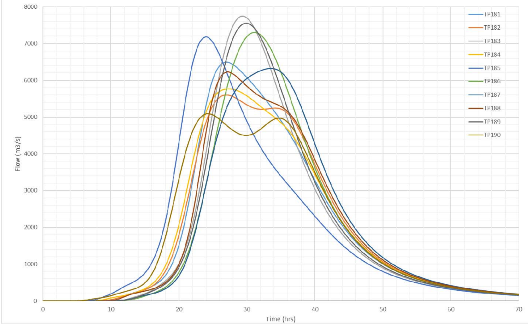
Figure 6 1% AEP IFD Comparison at Macquarie Grove
